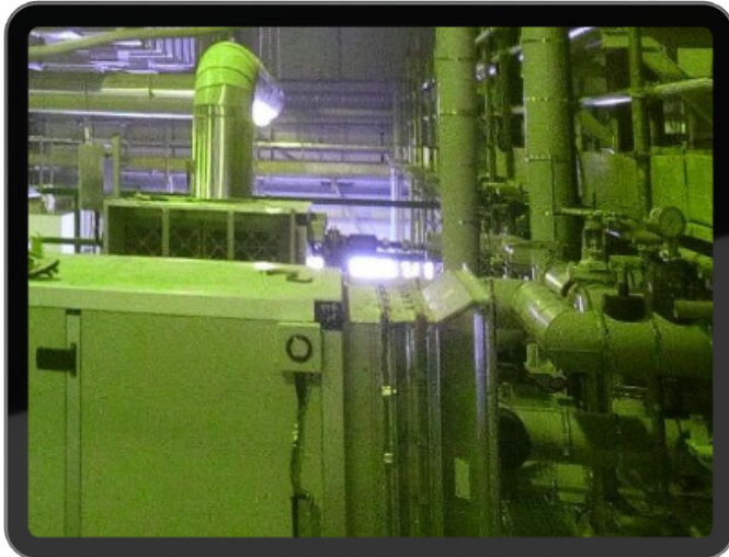
CHILLED WATER PIPING & CHILLER INSTALLED AT KEMYA SITE
